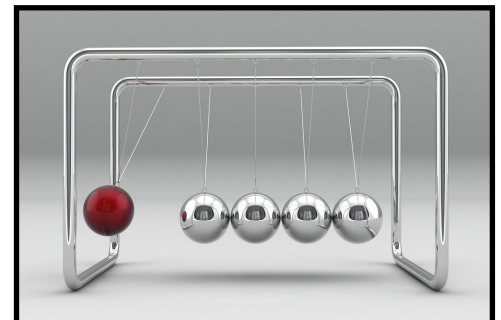
Newton's cradle
